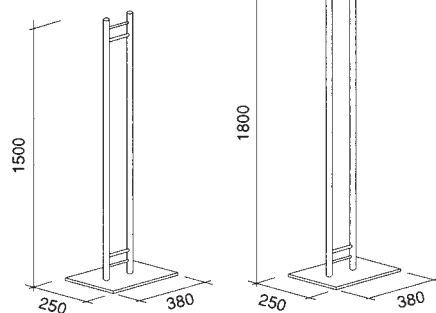
柱 A H1500 SR-1
