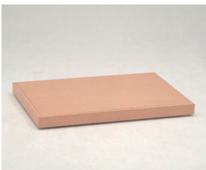
5 BST-1AK × 1 天板 (W.880 × D.580 × 12t) BST-1BK × 1 枠 (W.900 × D.600 × H60)
